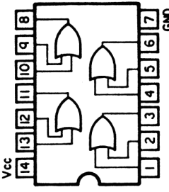
M74LS32P
