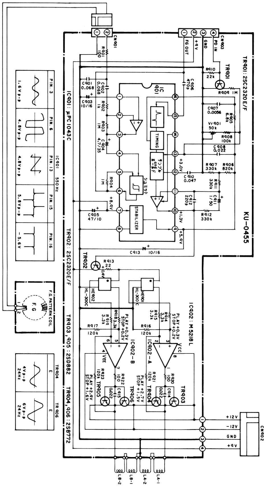
SCHEMATIC DIAGRAM OF CAPSTAN SERVO UNIT
