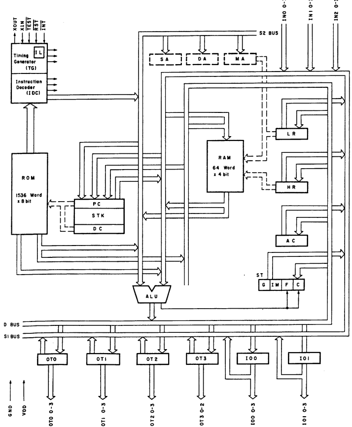
Fig. 8.1.11 4-Bit Micro-processor TMP4315BP-1814
