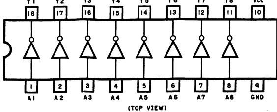
Fig. 8.1.9 FL Display Tube Driver LB1240
