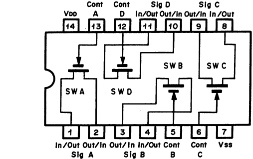
Fig. 8.1.6 Bilateral Switch C-MOS IC \mu PD4066BC
